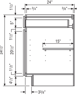
BASE CABINET
