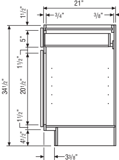
VANITY BASE 34 1/2" HIGH
