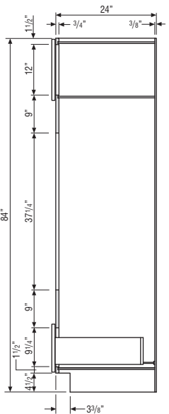
OVEN CABINET DOUBLE with DEEP DRAWER
