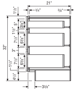
VANITY BASE THREE DRAWER 32" HIGH
