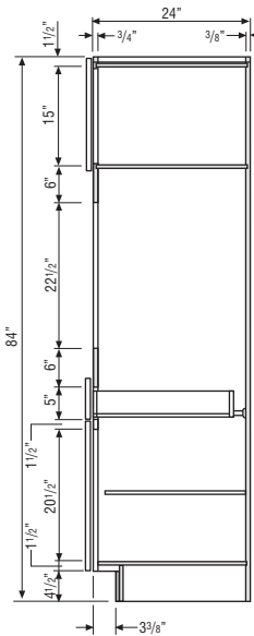
OVEN CABINET SINGLE
