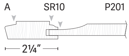
▼ Indicates Profile Glaze Locations
