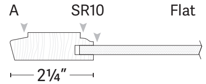
▼ Indicates Profile Glaze Locations
