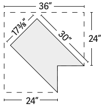
3DSCB TOP VIEW:
