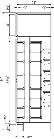
PANTRY CABINET
