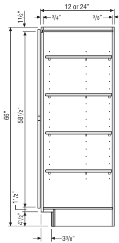
UTILITY CABINET
