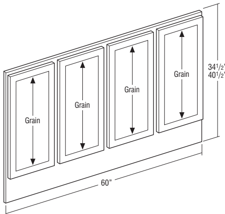
WAIN6034.5-WAIN6040.5
