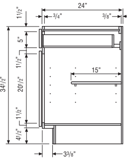
BASE CABINET
